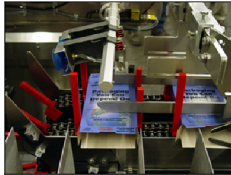
Jones Legend® Series L200 Cartoner
