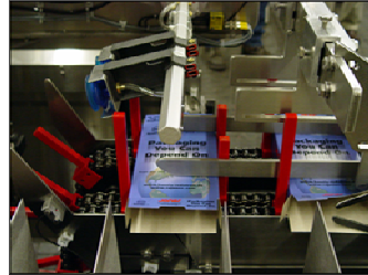
Jones Legend® Series L200 Cartoner System
